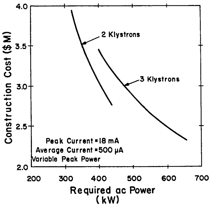
Fig. 7. DTL construction cost versus operating power requirement.
